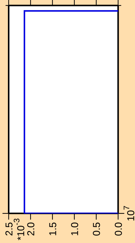
\Delta\sigma/\sigma vs. E for ^{125}\text{I}(\text{n},\text{pd})
