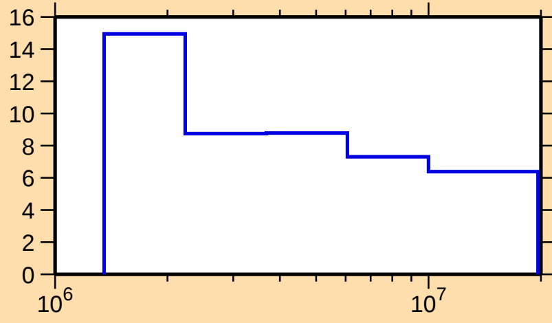
\Delta\sigma/\sigma vs. E for ^{125}\text{I}(\text{n},\text{nonel.})
