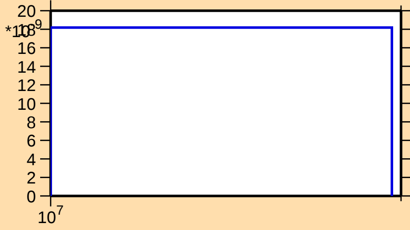
\sigma vs. E for ^{125}\text{I}(\text{n},\text{nd})
