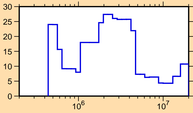
\Delta\sigma/\sigma vs. E for ^{126}\text{I}(n,el.)
