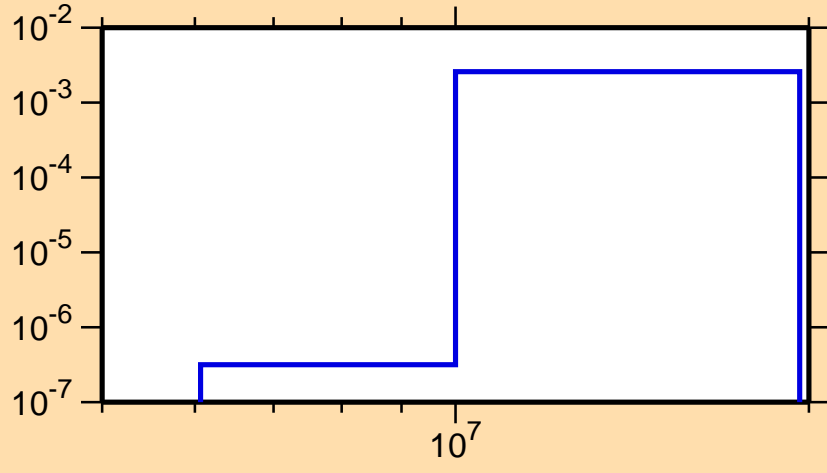
\sigma vs. E for ^{126}\text{I}(n,d)
