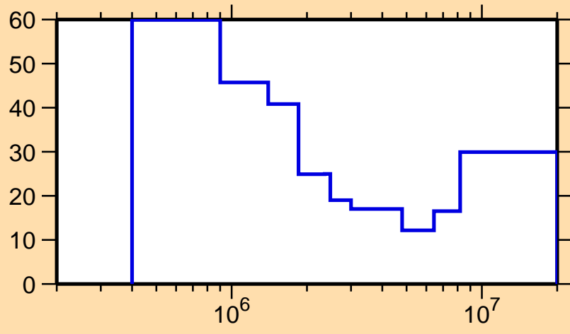
\Delta\sigma/\sigma vs. E for ^{126}\text{I}(n,n\text{cont.})
