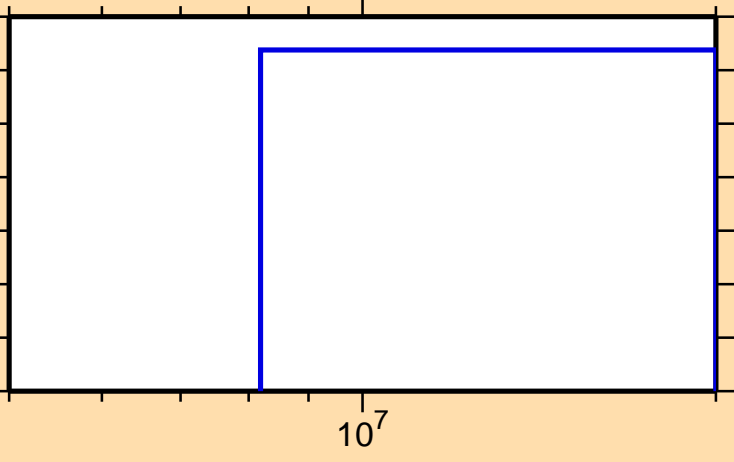
\sigma vs. E for ^{126}\text{I} (mt 34)
