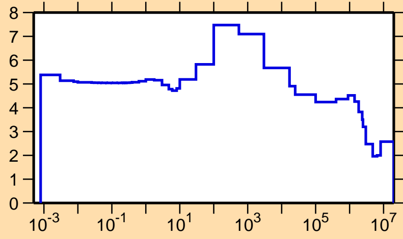
\sigma vs. E for ^{126}\text{I}(n,\text{el.})
