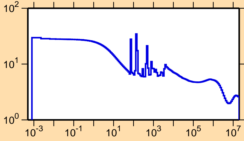
\sigma vs. E for ^{129}\text{I}(n,\text{el.})
