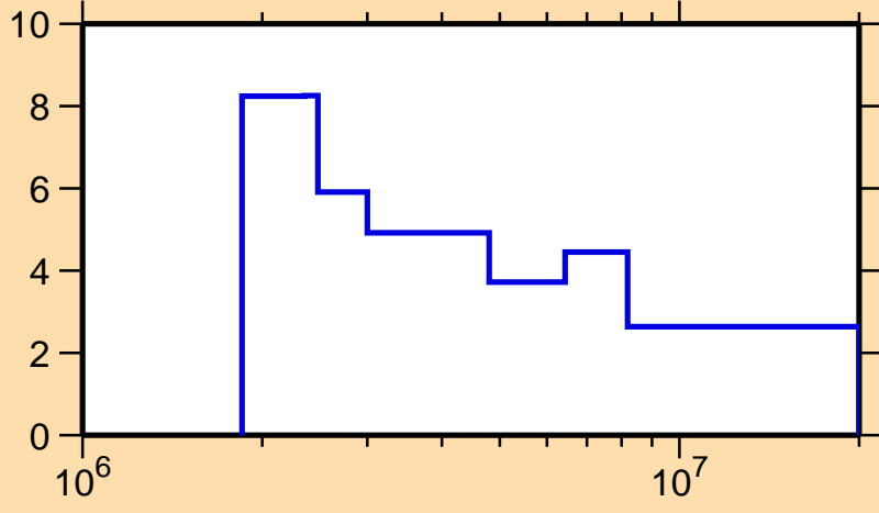
\Delta\sigma/\sigma vs. E for ^{129}\text{I}(n, tot.)
