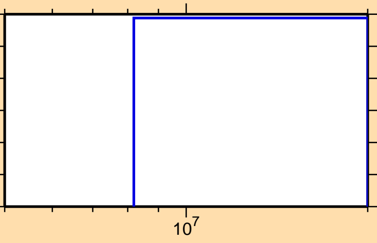
\sigma vs. E for ^{130}\text{I}(n,3n)
