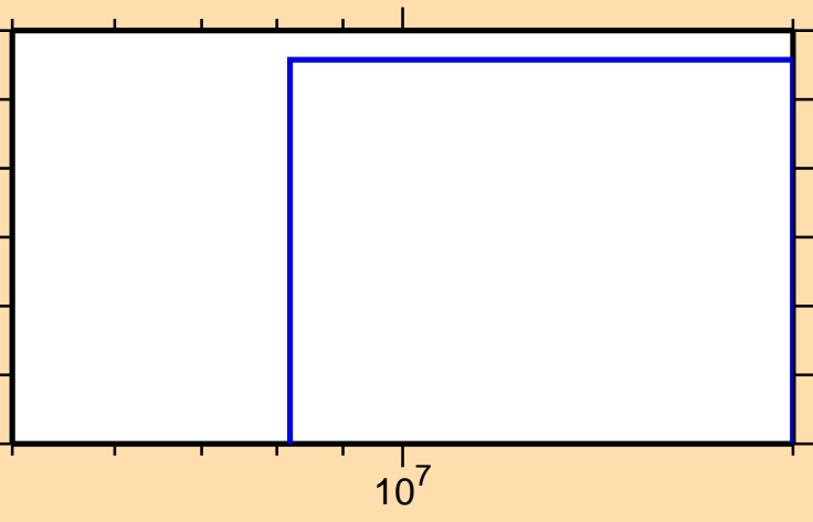
\sigma vs. E for ^{130}\text{I}(n,n\alpha)
