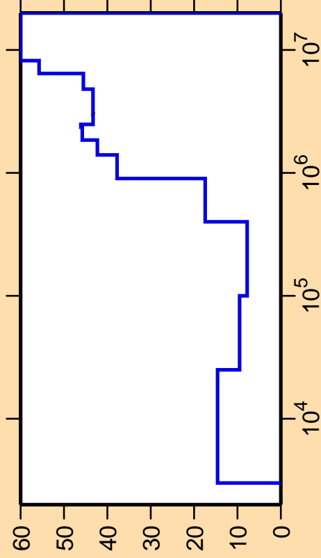
\Delta\sigma/\sigma vs. E for ^{130}\text{I}(n,n_3)
