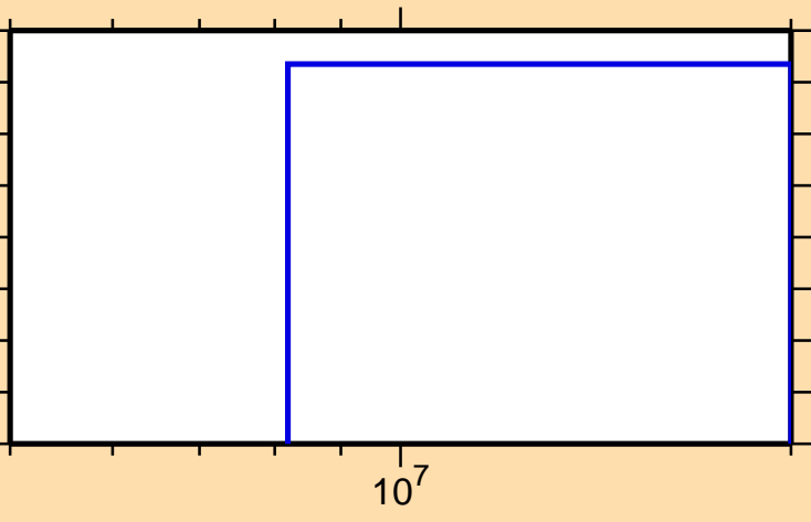
\sigma vs. E for ^{130}\text{I}(n,2np)
