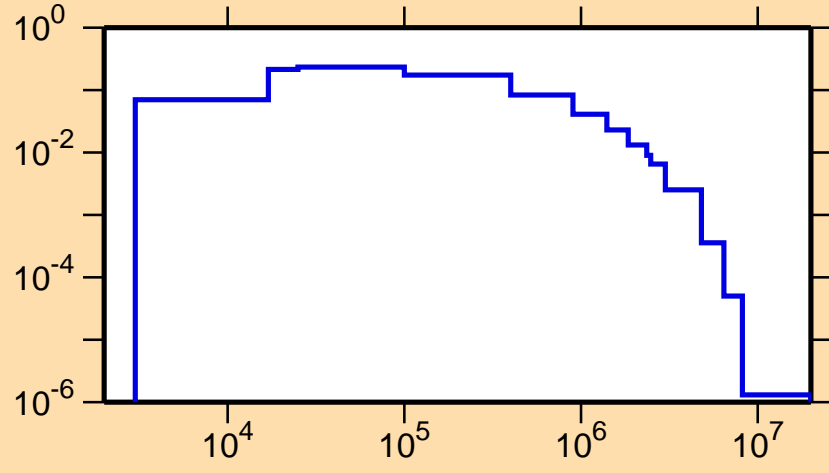
\sigma vs. E for ^{130}\text{I}(n,n_3)
