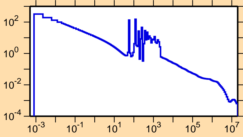
\sigma vs. E for ^{131}\text{I}(n,\gamma)
