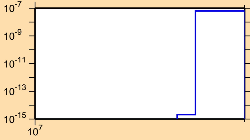
\sigma vs. E for ^{131}\text{I}(n,2np)
