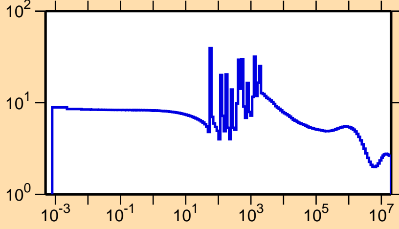
\sigma vs. E for ^{131}\text{I}(n,\text{el.})
