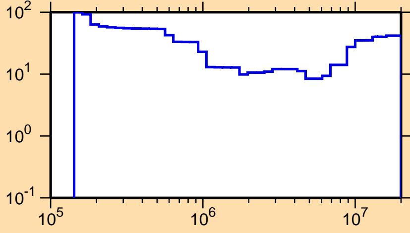
\Delta\sigma/\sigma vs. E for ^{131}\text{I}(n,\text{inel.})
