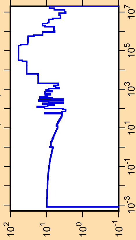
\Delta\sigma/\sigma vs. E for ^{131}\text{I}(n,\text{tot.})
