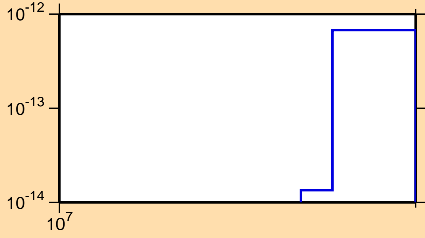
\sigma vs. E for ^{131}\text{I}(n,p\alpha)
