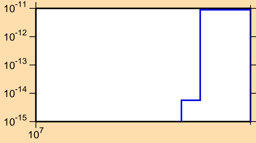
\sigma vs. E for ^{131}\text{I}(n,\text{He}3)
