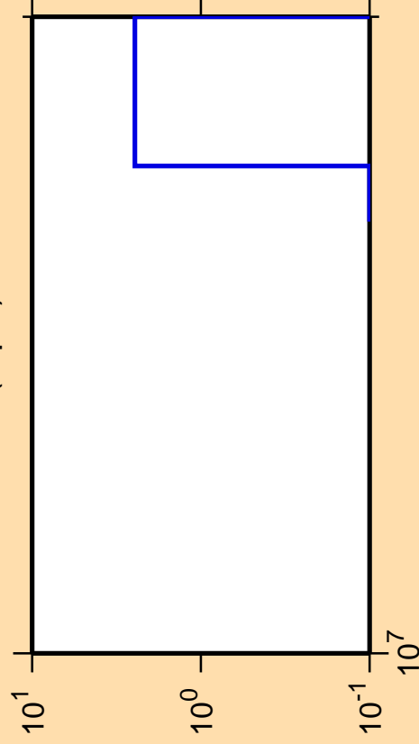
\Delta\sigma/\sigma vs. E for ^{131}\text{I}(n,p\alpha)
