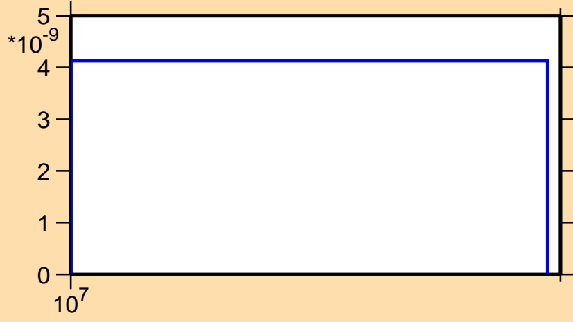
\sigma vs. E for ^{131}\text{I}(n,nd)
