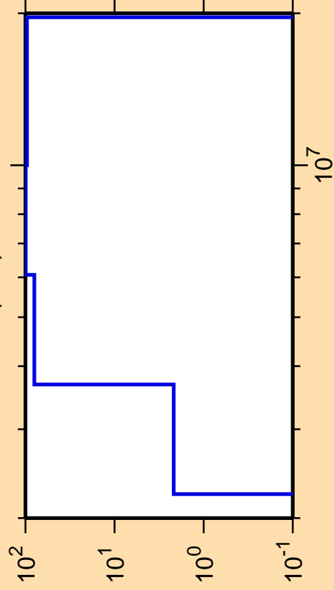
\Delta\sigma/\sigma vs. E for ^{131}\text{I}(n,\alpha)
