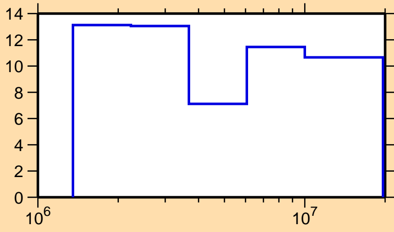
\Delta\sigma/\sigma vs. E for ^{131}\text{I}(n, el.)
