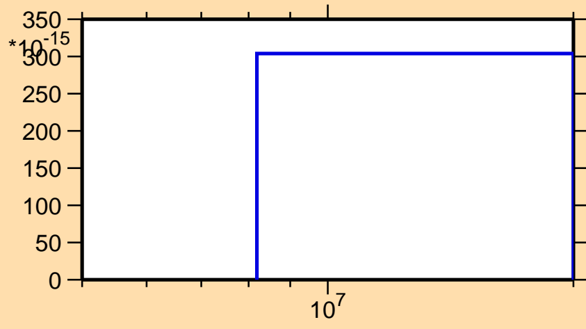
\sigma vs. E for ^{131}\text{I}(n,2n\alpha)
