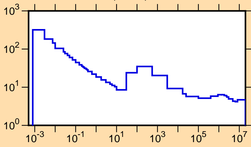
\sigma vs. E for ^{131}\text{I}(n,\text{tot.})
