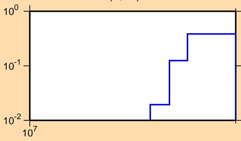
\sigma vs. E for ^{132}\text{I}(n,3n)
