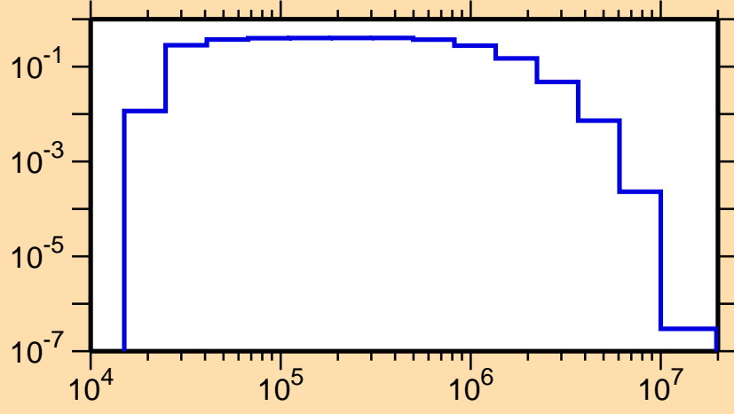
\sigma vs. E for ^{132}\text{I}(n,n_1)
