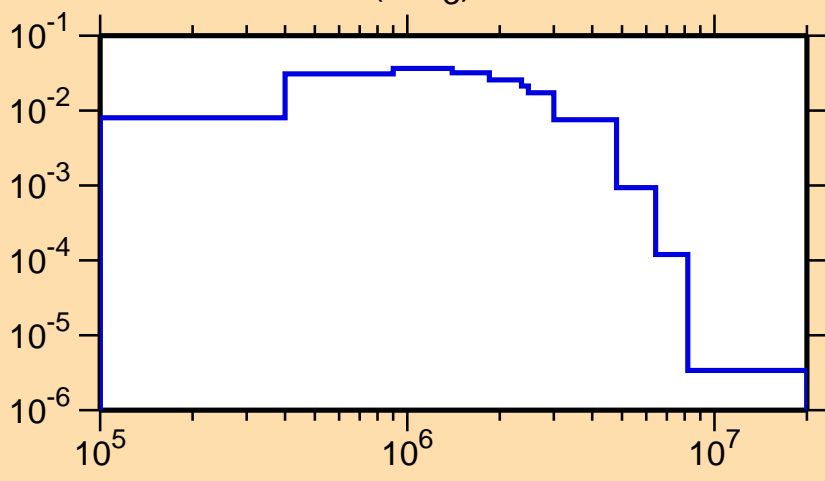
\sigma vs. E for ^{132}\text{I}(n,n_3)
