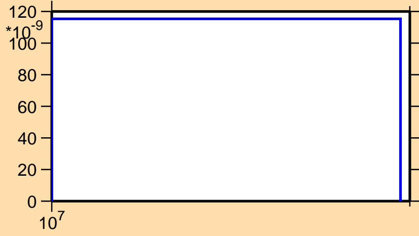
\sigma vs. E for ^{132}\text{I}(n,nd)
