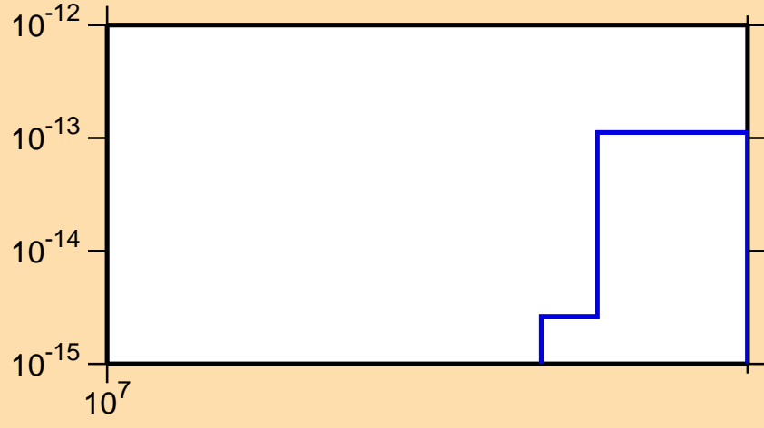
\sigma vs. E for ^{133}\text{I}(n,p\alpha)
