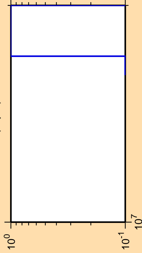
\Delta\sigma/\sigma vs. E for ^{133}\text{I}(n,p\alpha)
