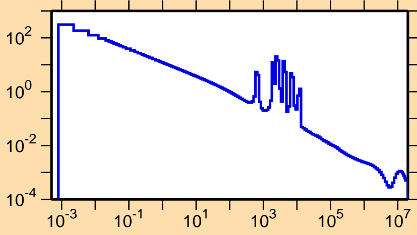
\sigma vs. E for ^{133}\text{I}(n,\gamma)
