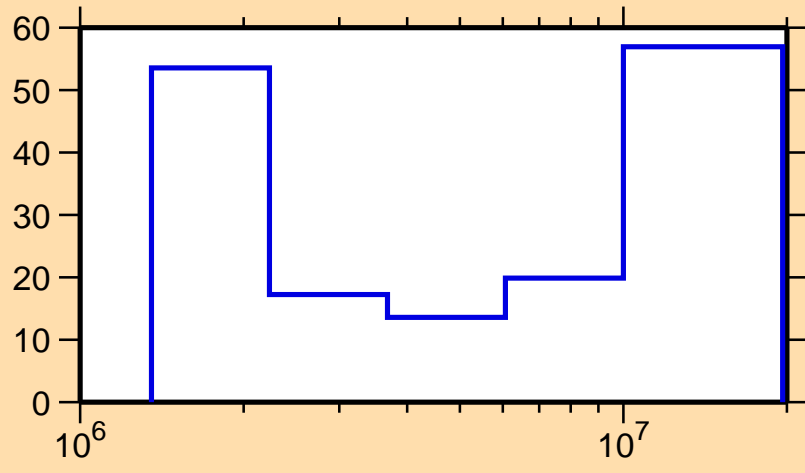
\Delta\sigma/\sigma vs. E for ^{133}\text{I}(n,n\text{cont.})
