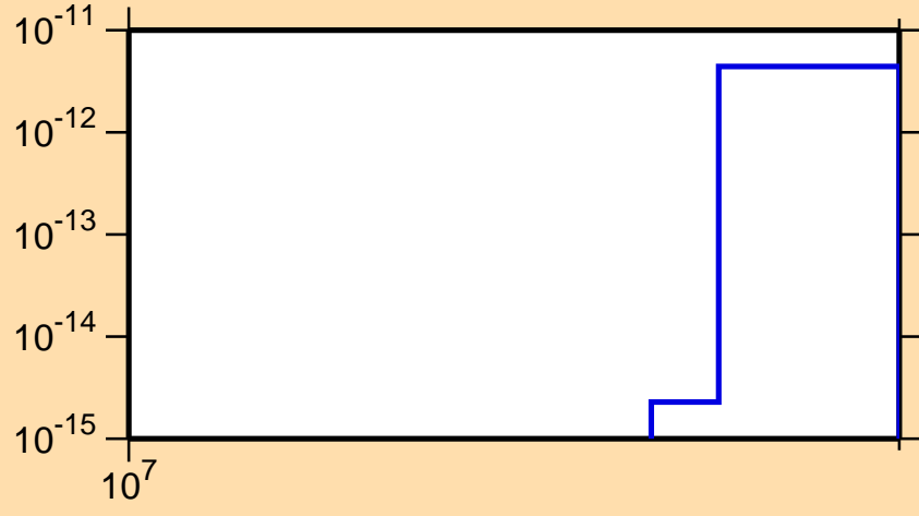
\sigma vs. E for ^{134}\text{I}(n,\text{He}3)
