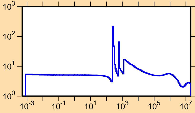
\sigma vs. E for ^{134}\text{I}(n,\text{el.})
