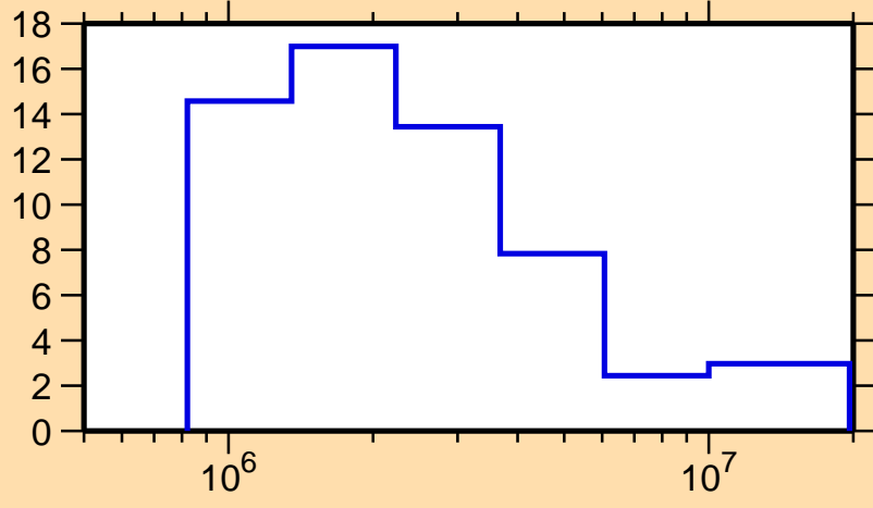
\Delta\sigma/\sigma vs. E for ^{134}\text{I}(n, tot.)
