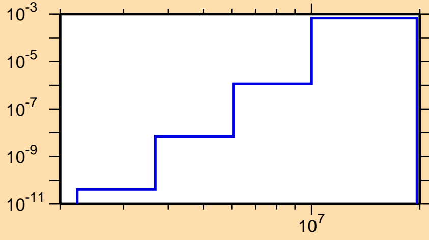
\sigma vs. E for ^{134}\text{I}(n,\alpha)
