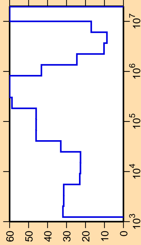
\Delta\sigma/\sigma vs. E for ^{134}\text{I}(n,\text{inel.})
