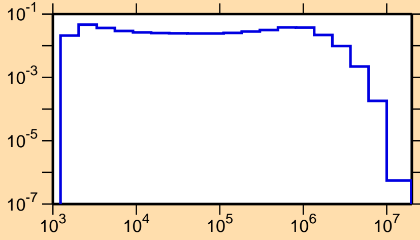
\sigma vs. E for ^{134}\text{I}(n,n_1)
