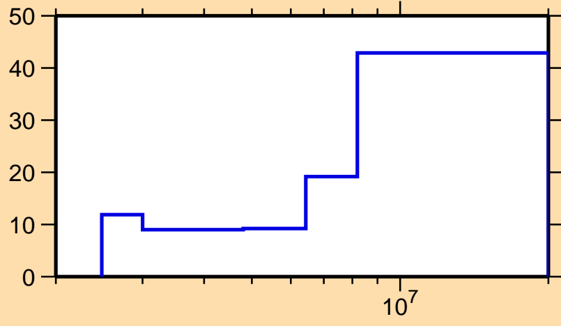
\Delta\sigma/\sigma vs. E for ^{134}\text{I}(n,n\text{cont.})
