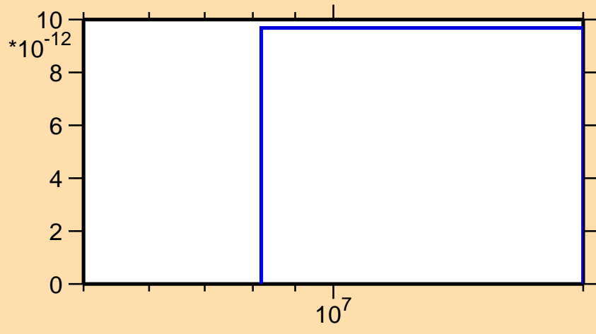
\sigma vs. E for ^{134}\text{I}(n,2n\alpha)
