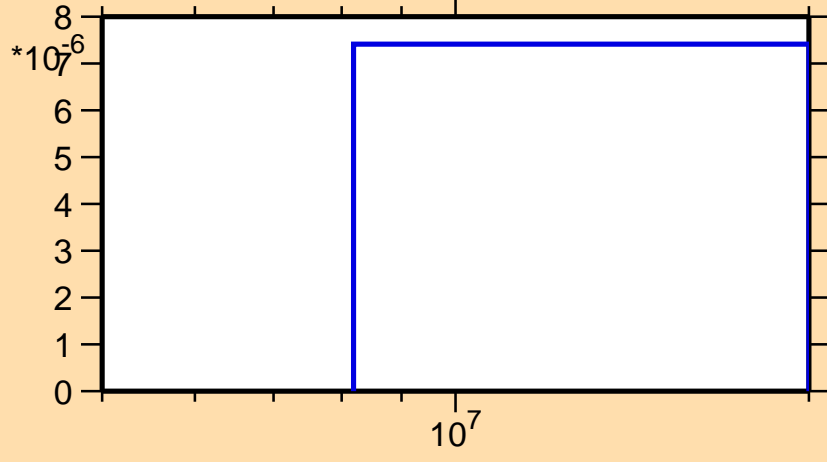
\sigma vs. E for ^{134}\text{I}(n,n\alpha)
