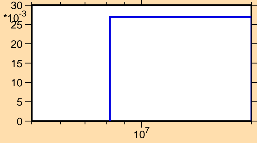
\sigma vs. E for ^{134}\text{I}(n,3n)
