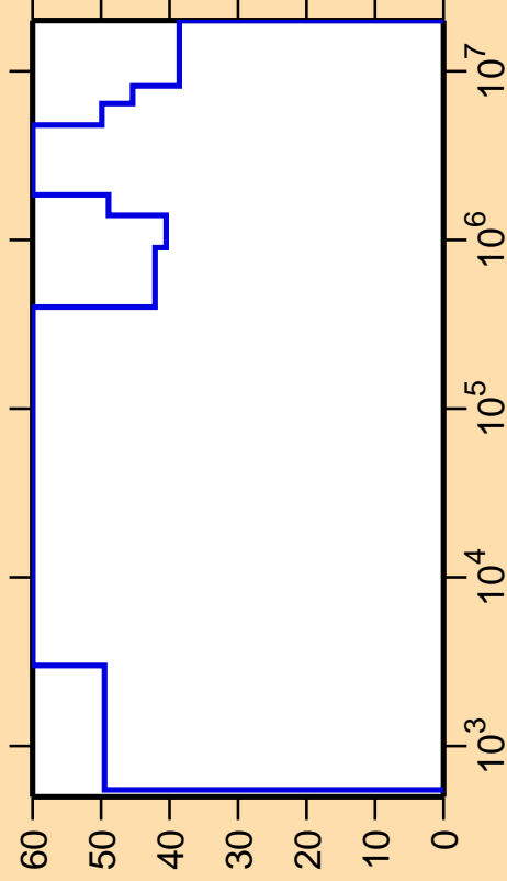
\Delta\sigma/\sigma vs. E for ^{134}\text{I}(n,n_2)
