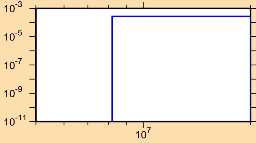
\sigma vs. E for ^{134}\text{I}(n,np)
