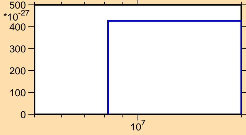
\sigma vs. E for ^{134}\text{I} (mt 11)
