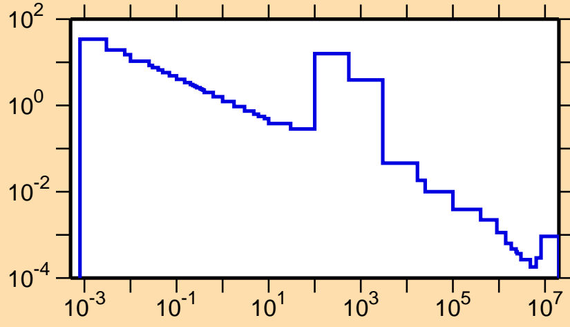
\sigma vs. E for ^{134}\text{I}(n,\gamma)
