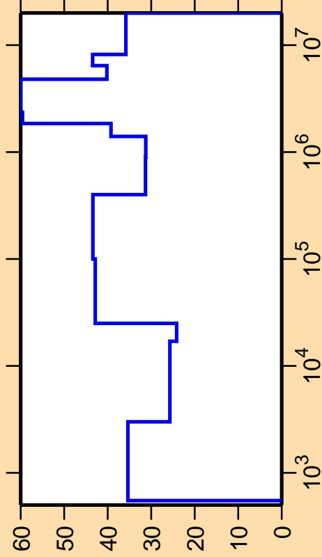
\Delta\sigma/\sigma vs. E for ^{134}\text{I}(n,n_1)
