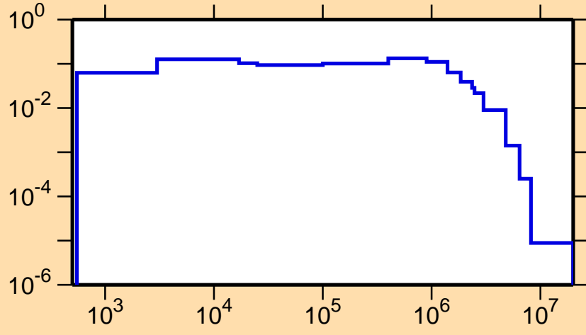
\sigma vs. E for ^{134}\text{I}(n,n_2)
