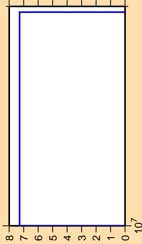
\Delta\sigma/\sigma vs. E for ^{135}\text{I}(n,2np)
