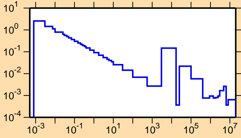
\sigma vs. E for ^{135}\text{I}(n,\gamma)
