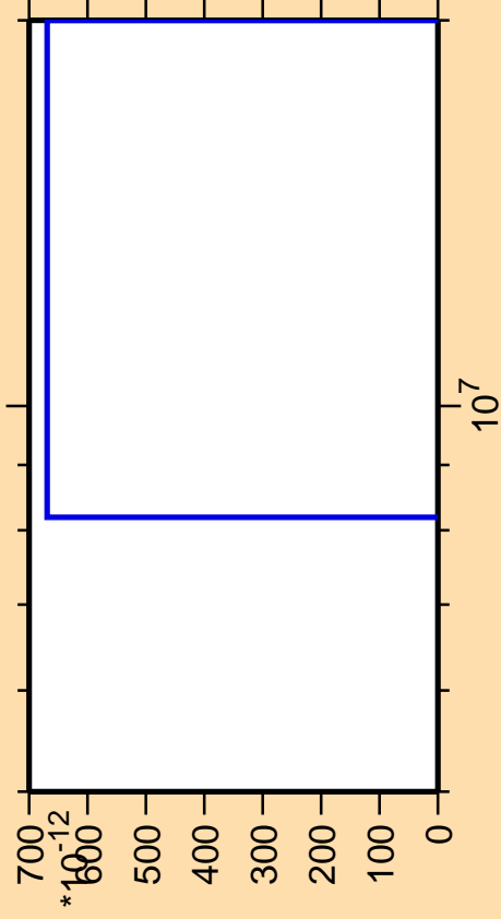
\Delta\sigma/\sigma vs. E for ^{135}\text{I} (mt 11)
