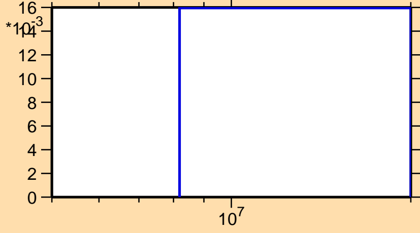
\sigma vs. E for ^{135}\text{I}(n,3n)
