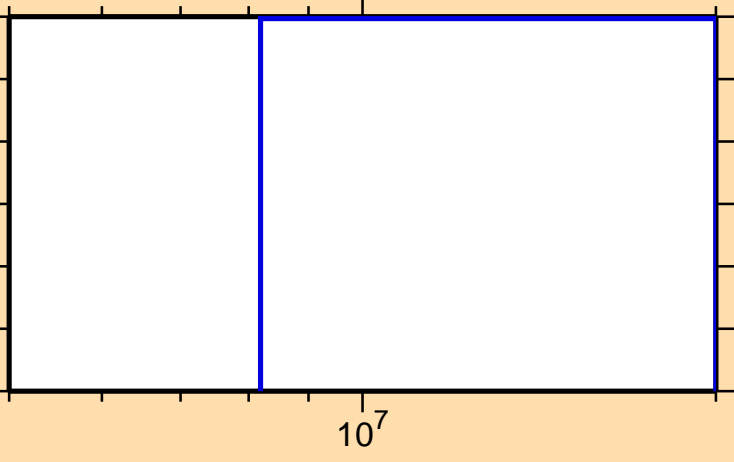
\sigma vs. E for ^{135}\text{I}(n,np)
