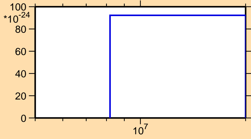
\sigma vs. E for ^{135}\text{I} (mt 11)
