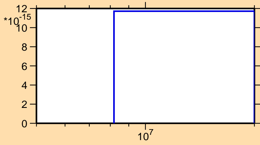
\sigma vs. E for ^{135}\text{I}(n,2n\alpha)
