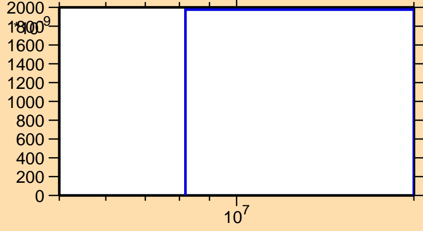
\sigma vs. E for ^{135}\text{I}(n,n\alpha)
