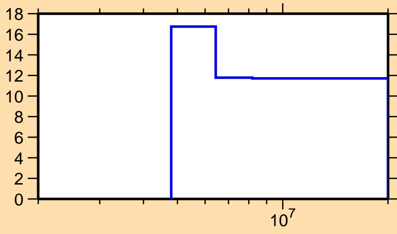
\Delta\sigma/\sigma vs. E for ^{135}\text{I}(n, n\text{onel.})
