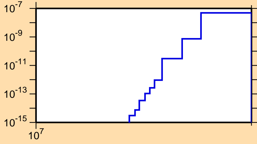
\sigma vs. E for ^{136}\text{I}(n,2n\alpha)
