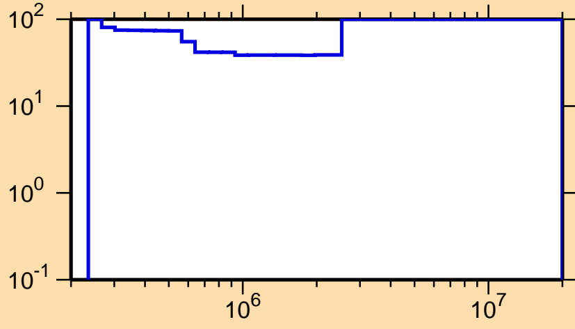
\Delta\sigma/\sigma vs. E for ^{136}\text{I}(n,n_1)
