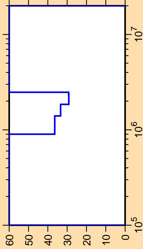
\Delta\sigma/\sigma vs. E for ^{136}\text{I}(n,n_3)
