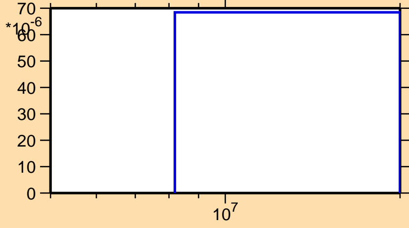
\sigma vs. E for ^{136}\text{I}(n,np)
