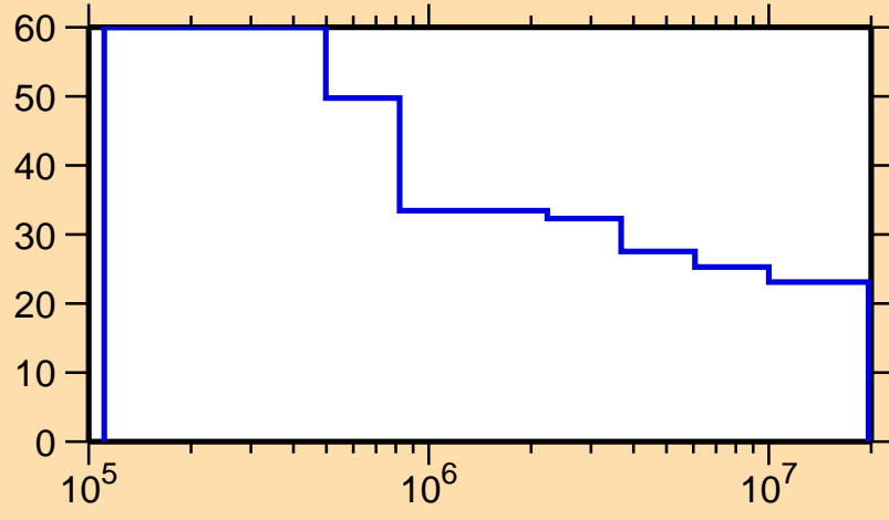
\Delta\sigma/\sigma vs. E for ^{136}\text{I}(n,\text{nonel.})
