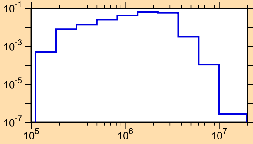
\sigma vs. E for ^{136}\text{I}(n,n_3)
