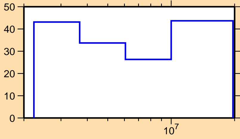
\Delta\sigma/\sigma vs. E for ^{136}\text{I}(n,2n)
