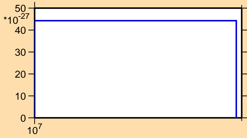
\sigma vs. E for ^{136}\text{I} (mt 42)
