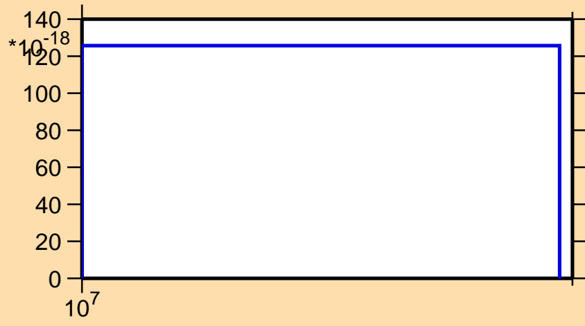
\sigma vs. E for ^{136}\text{I} (mt 11)
