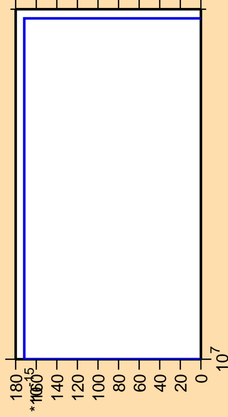
\Delta\sigma/\sigma vs. E for ^{136}\text{I} (mt 42)
