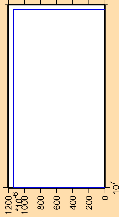
\Delta\sigma/\sigma vs. E for ^{136}\text{I} (mt 11)
