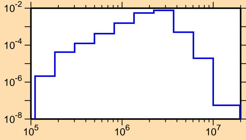
\sigma vs. E for ^{136}\text{I}(n,n_2)
