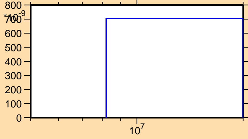
\sigma vs. E for ^{136}\text{I}(n,nt)
