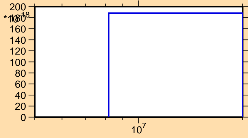
\sigma vs. E for ^{136}\text{I}(\text{mt } 11)
