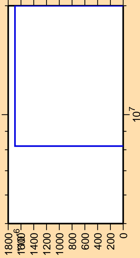
\Delta\sigma/\sigma vs. E for ^{136}\text{I}(\text{mt } 11)
