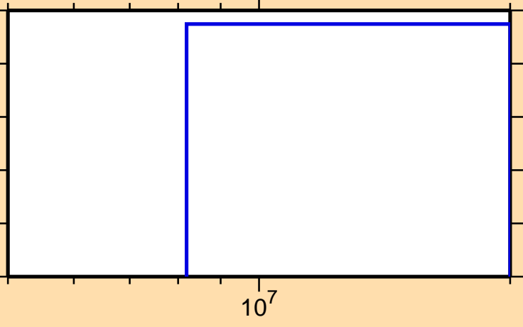
\sigma vs. E for ^{136}\text{I}(n,\text{nd})
