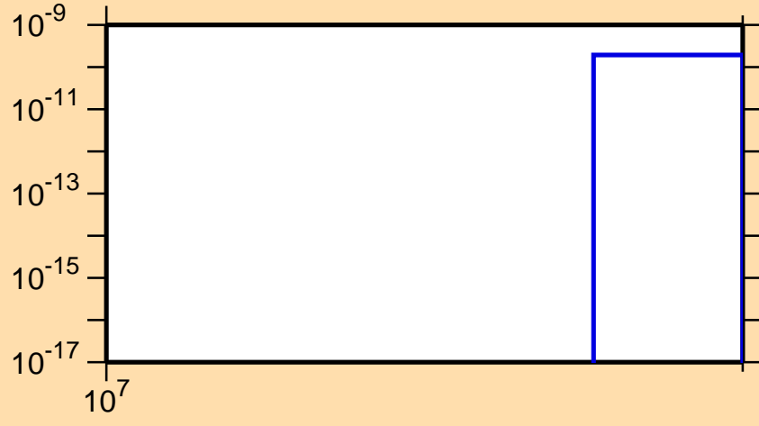
\sigma vs. E for ^{138}\text{I} (mt 11)
