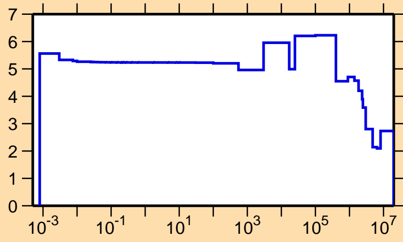
\sigma vs. E for ^{138}\text{I}(n,\text{el.})
