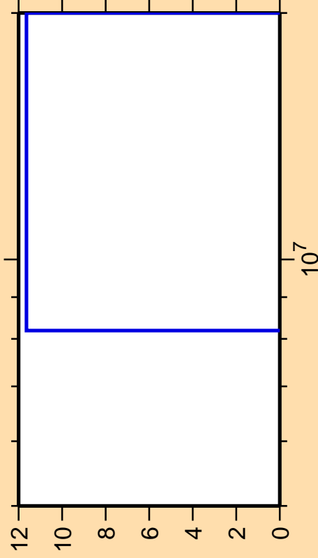
\Delta\sigma/\sigma vs. E for ^{138}\text{I}(\text{mt } 11)
