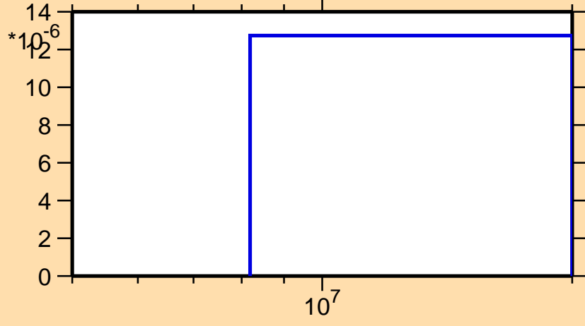
\sigma vs. E for ^{138}\text{I}(n,nt)
