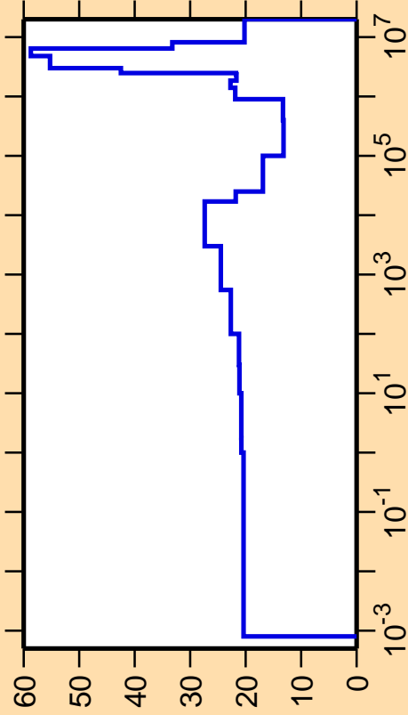
\Delta\sigma/\sigma vs. E for ^{138}\text{I}(n,\text{el.})
