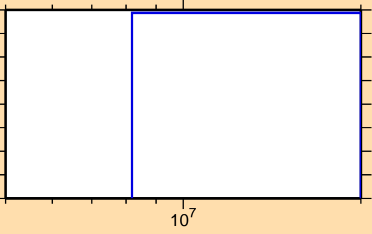
\sigma vs. E for ^{138}\text{I}(n,np)
