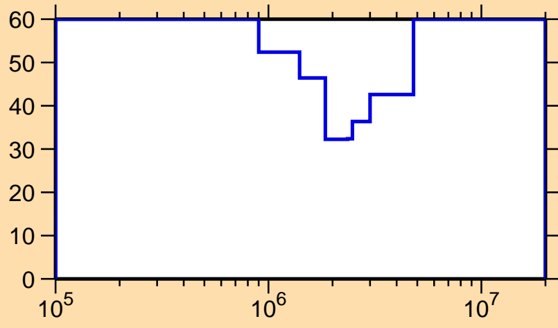
\Delta\sigma/\sigma vs. E for ^{138}\text{I}(n,n\text{cont.})
