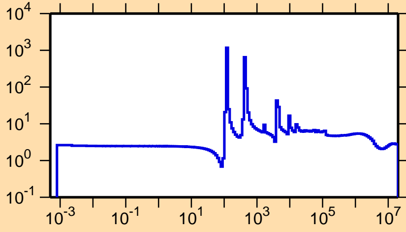
\sigma vs. E for ^{139}\text{I}(n,\text{el.})
