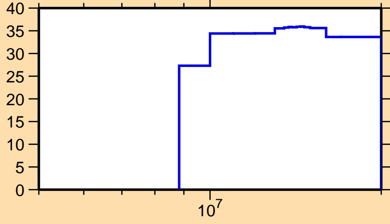
\Delta\sigma/\sigma vs. E for ^{139}\text{I}(n,2n)
