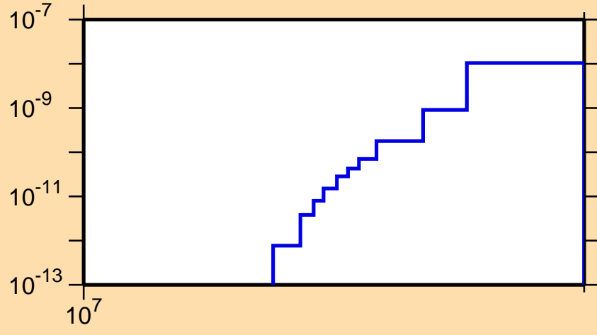
\sigma vs. E for ^{139}\text{I}(n,3n\alpha)
