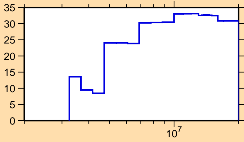
\Delta\sigma/\sigma vs. E for ^{139}\text{I}(n,n\text{cont.})
