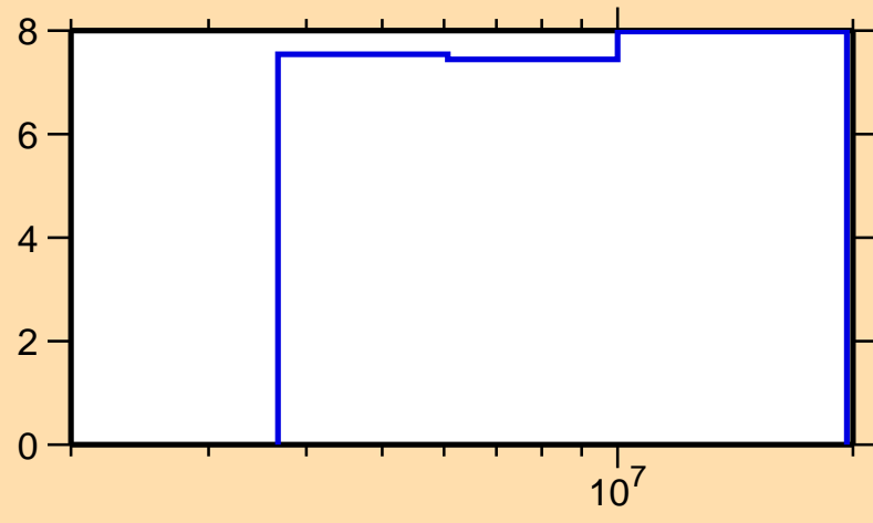
\Delta\sigma/\sigma vs. E for ^{139}\text{I}(n,\text{nonel.})
