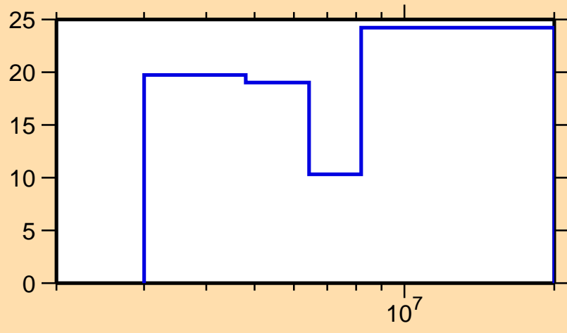
\Delta\sigma/\sigma vs. E for ^{139}\text{I}(n,2n)
