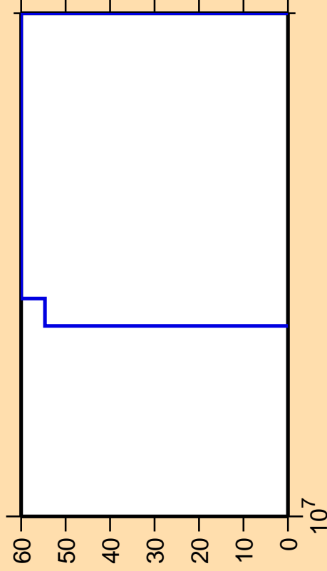
\Delta\sigma/\sigma vs. E for ^{98}\text{In}(n,nd)
