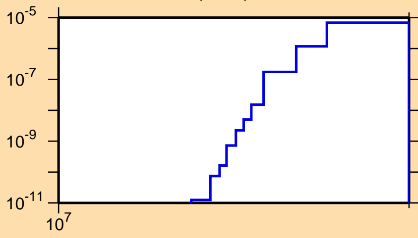
\sigma vs. E for ^{98}\text{In}(n,nd)
