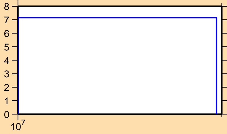
\Delta\sigma/\sigma vs. E for ^{98}\text{In}(n,\text{el.})
