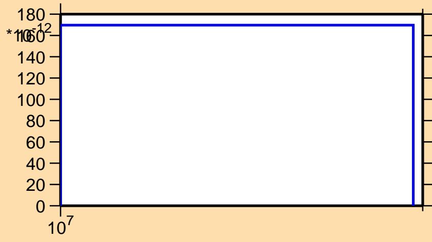
\sigma vs. E for ^{98}\text{In}(\text{mt } 34)
