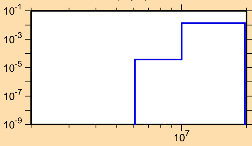
\sigma vs. E for ^{98}\text{In}(n,\text{pd})
