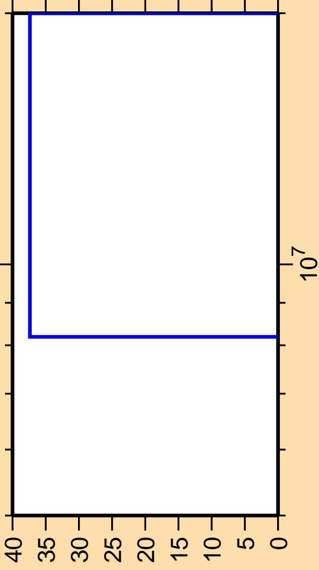
\Delta\sigma/\sigma vs. E for ^{98}\text{In}(n,p)
