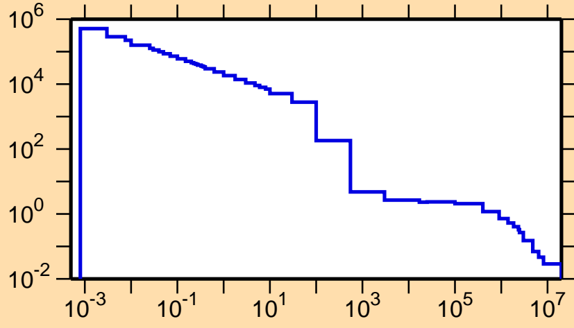
\sigma vs. E for ^{98}\text{In}(n,p)
