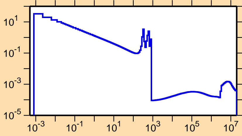
\sigma vs. E for ^{100}\text{In}(n,\gamma)
