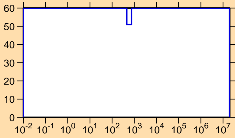
\Delta\sigma/\sigma vs. E for ^{100}\text{In}(n,\gamma)
