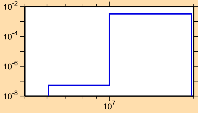
\sigma vs. E for ^{100}\text{In}(n,pd)
