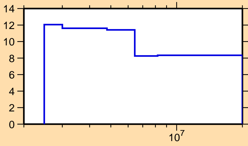
\Delta\sigma/\sigma vs. E for ^{100}\text{In}(n,\text{nonel.})
