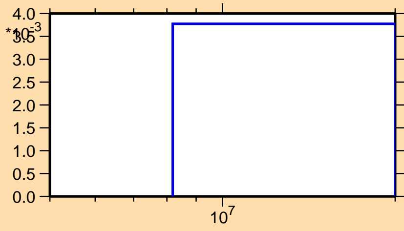
\sigma vs. E for ^{100}\text{In}(n,2n)
