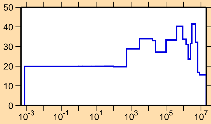
\Delta\sigma/\sigma vs. E for ^{100}\text{In}(n,el.)
