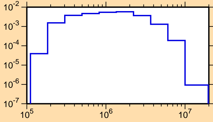
\sigma vs. E for ^{102}\text{In}(n,n_3)
