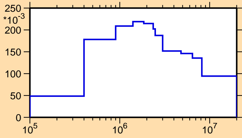
\sigma vs. E for ^{102}\text{In}(n,\text{inel.})
