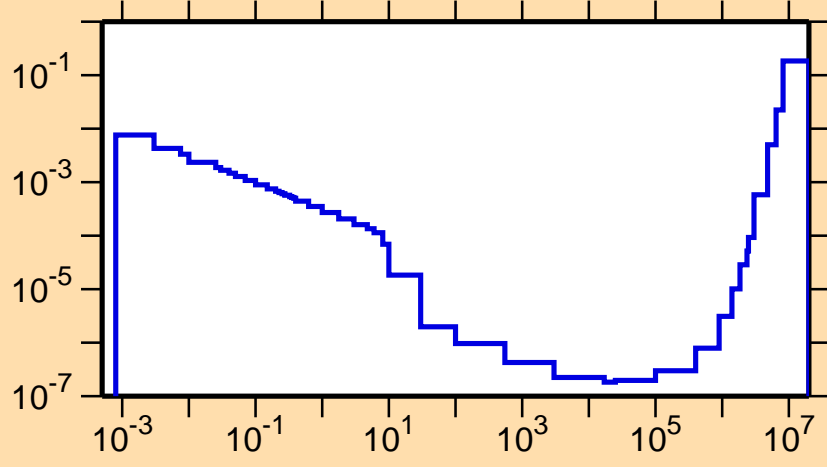
\sigma vs. E for ^{102}\text{In}(n,p)\alpha
