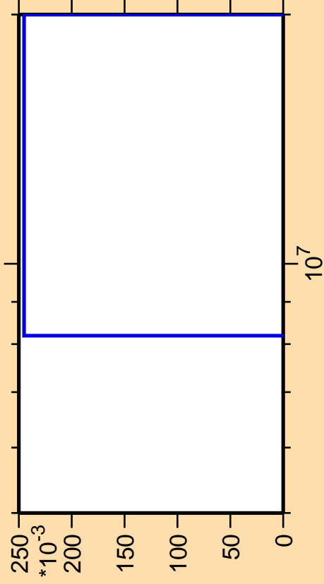
\Delta\sigma/\sigma vs. E for ^{102}\text{In}(n,nt)
