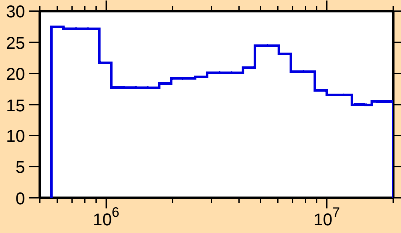
\Delta\sigma/\sigma vs. E for ^{103}\text{In}(\text{n,nonel.})
