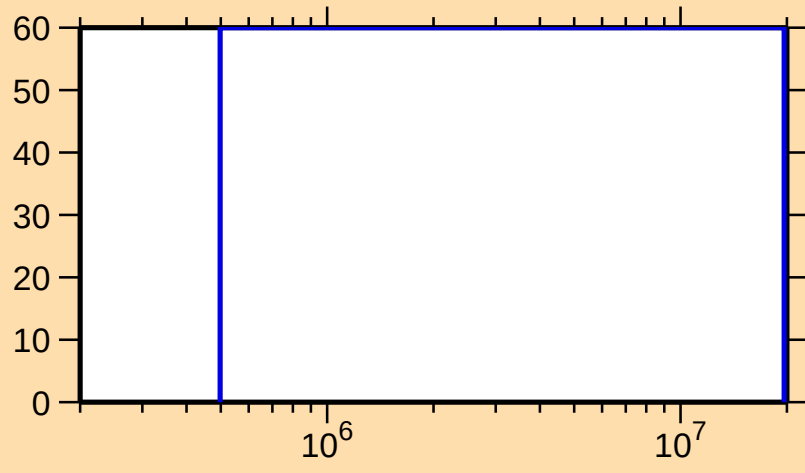
\Delta\sigma/\sigma vs. E for ^{103}\text{In}(n, n_1)
