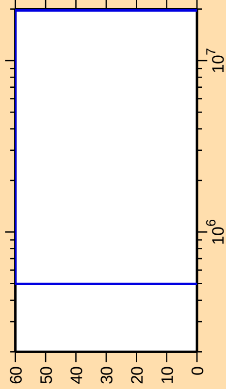
\Delta\sigma/\sigma vs. E for ^{103}\text{In}(\alpha, n)
