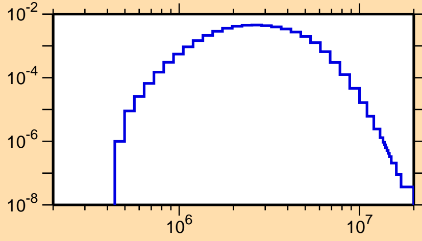
\sigma vs. E for ^{103}\text{In}(n,n_2)
