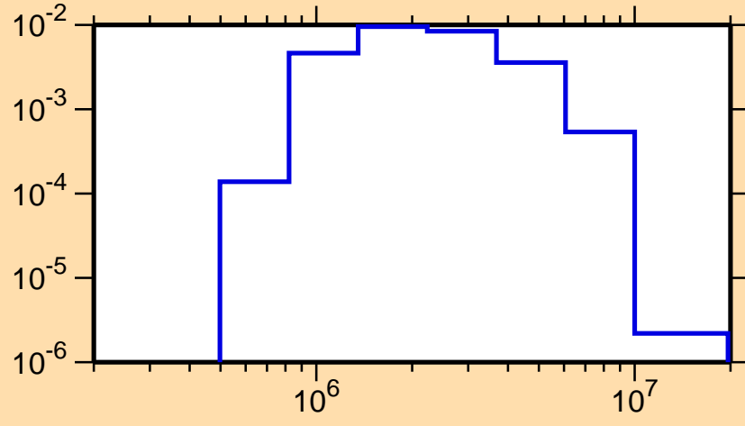
\sigma vs. E for ^{103}\text{In}(n,n_4)
