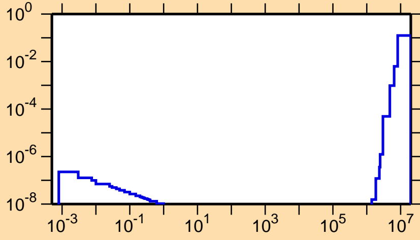
\sigma vs. E for ^{103}\text{In}(n,p\alpha)
