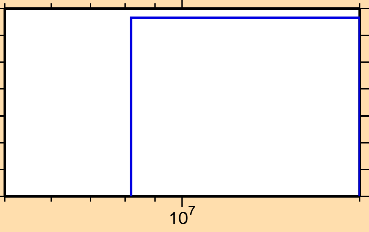
\sigma vs. E for ^{103}\text{In}(n,nd)
