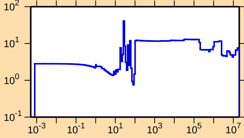
\Delta\sigma/\sigma vs. E for ^{104}\text{In}(n,\text{el.})
