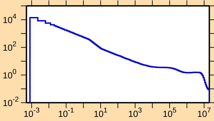
\sigma vs. E for ^{104}\text{In}(n,p)
