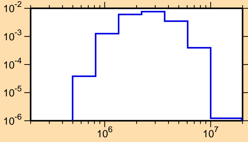
\sigma vs. E for ^{105}\text{In}(n,n_4)
