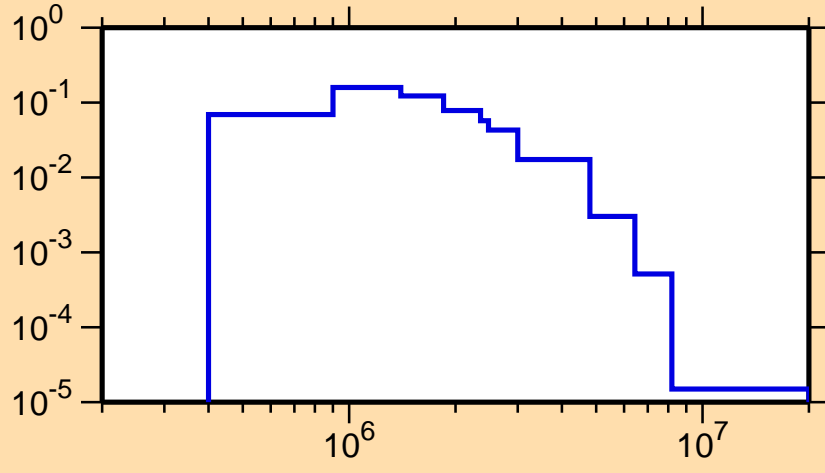
\sigma vs. E for ^{105}\text{In}(n,n_3)
