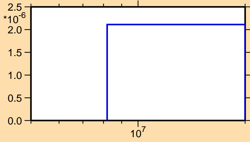
\sigma vs. E for ^{105}\text{In}(n,nd)
