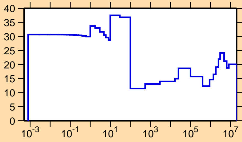
\Delta\sigma/\sigma vs. E for ^{105}\text{In}(n,el.)
