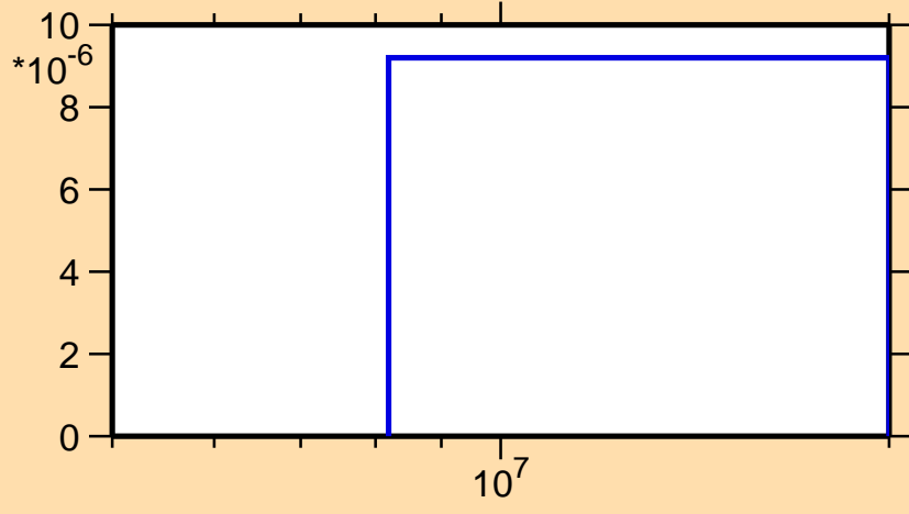
\sigma vs. E for ^{105}\text{In}(\text{mt } 45)
