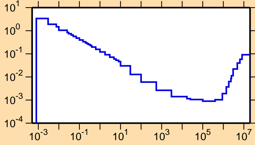
\sigma vs. E for ^{105}\text{In}(n,\alpha)
