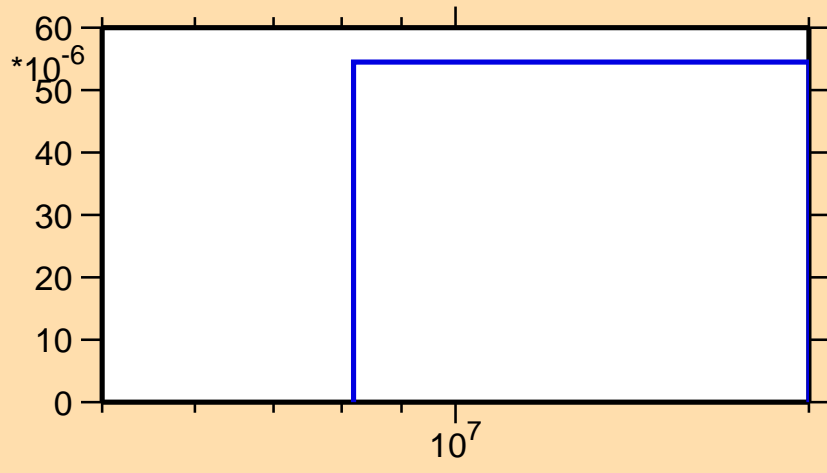
\sigma vs. E for ^{105}\text{In}(n,\text{pd})
