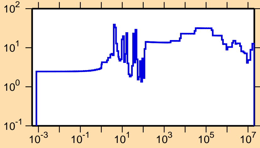
\Delta\sigma/\sigma vs. E for ^{106}\text{In}(n,el.)
