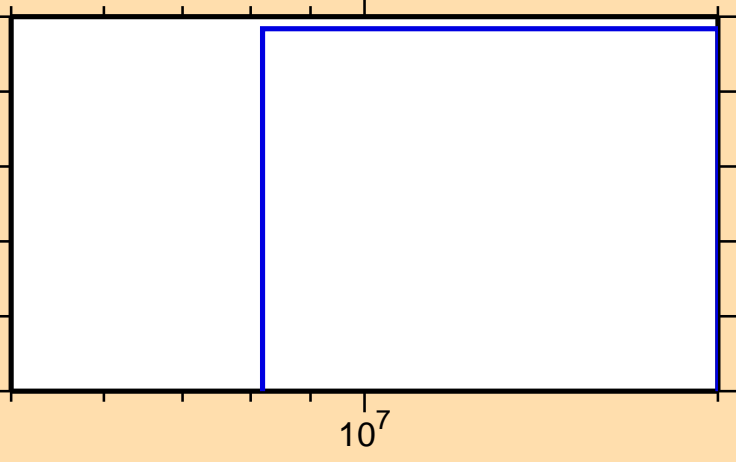
\sigma vs. E for ^{106}\text{In}(\text{mt117})
