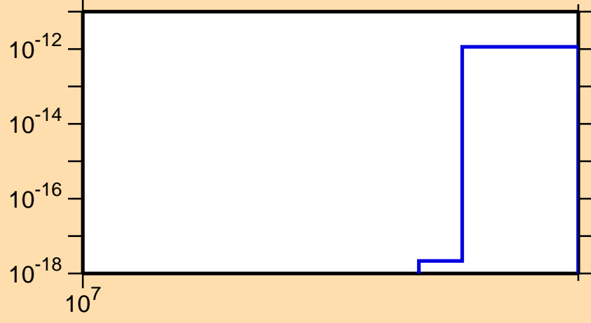
\sigma vs. E for ^{107}\text{In} (mt 34)
