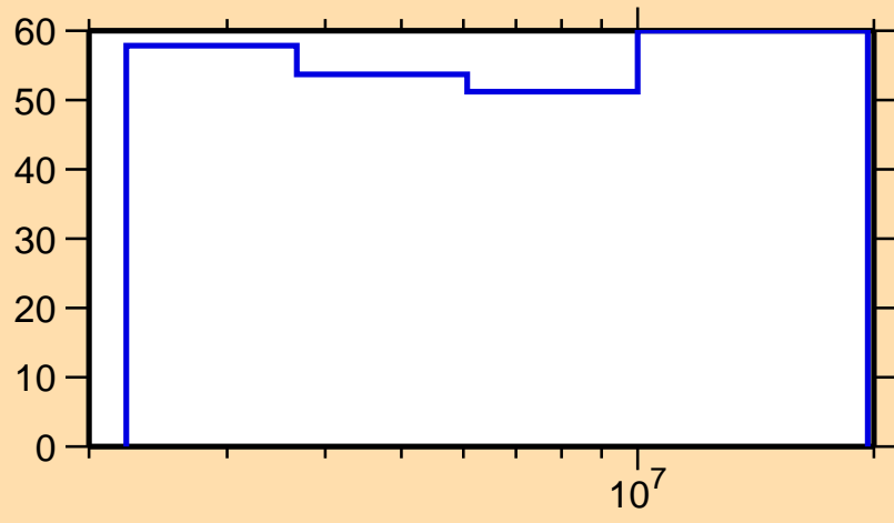
\Delta\sigma/\sigma vs. E for ^{107}\text{In}(n,n\text{cont.})
