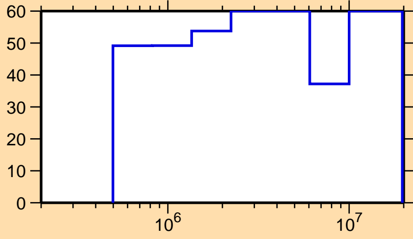
\Delta\sigma/\sigma vs. E for ^{107}\text{In}(n,n_1)
