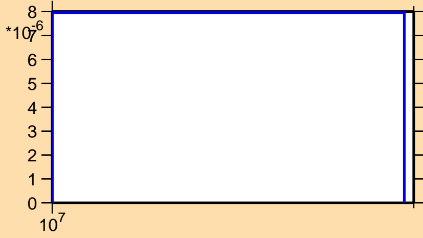
\sigma vs. E for ^{107}\text{In}(n,2np)
