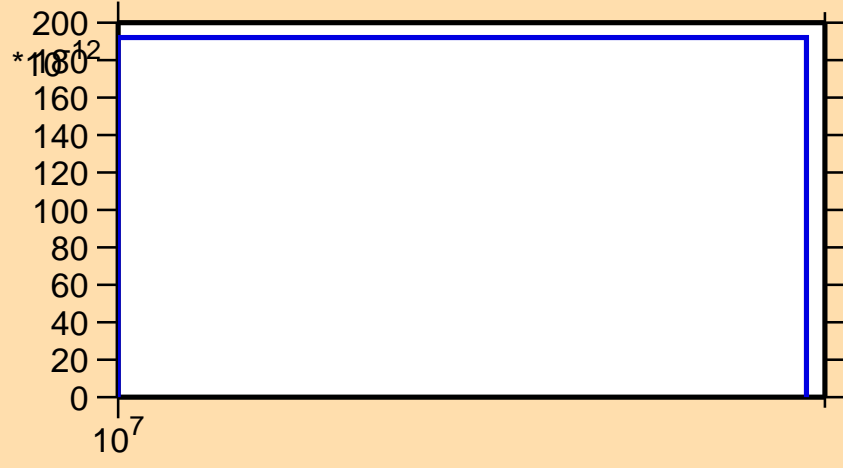
\sigma vs. E for ^{107}\text{In}(n,2n\alpha)
