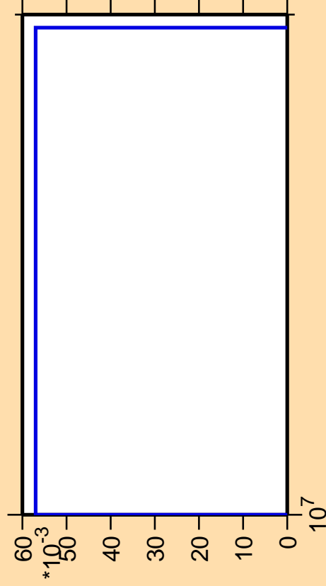
\Delta\sigma/\sigma vs. E for ^{107}\text{In}(\text{mt } 34)
