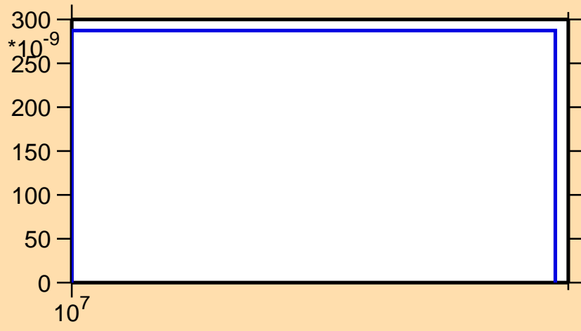
\sigma vs. E for ^{107}\text{In}(n,\text{nd})
